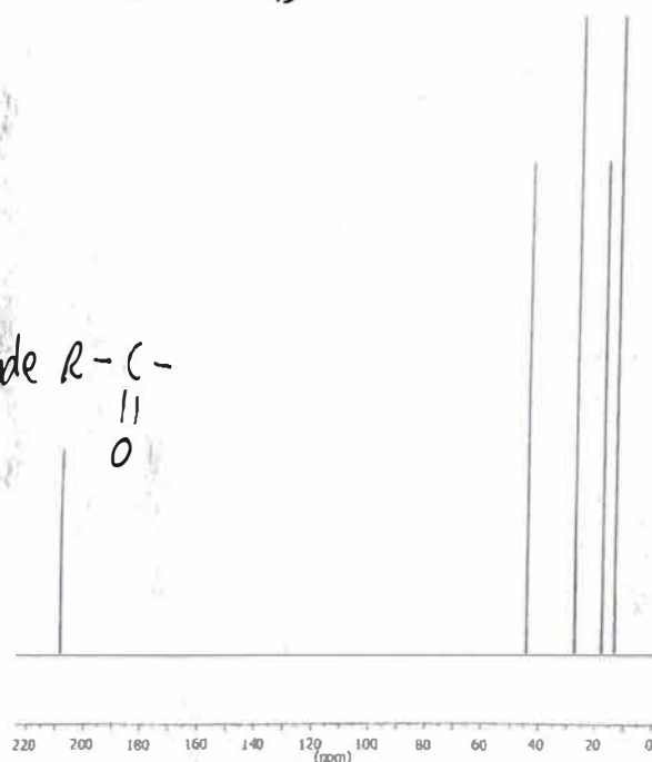
13 C NMR spectrum
