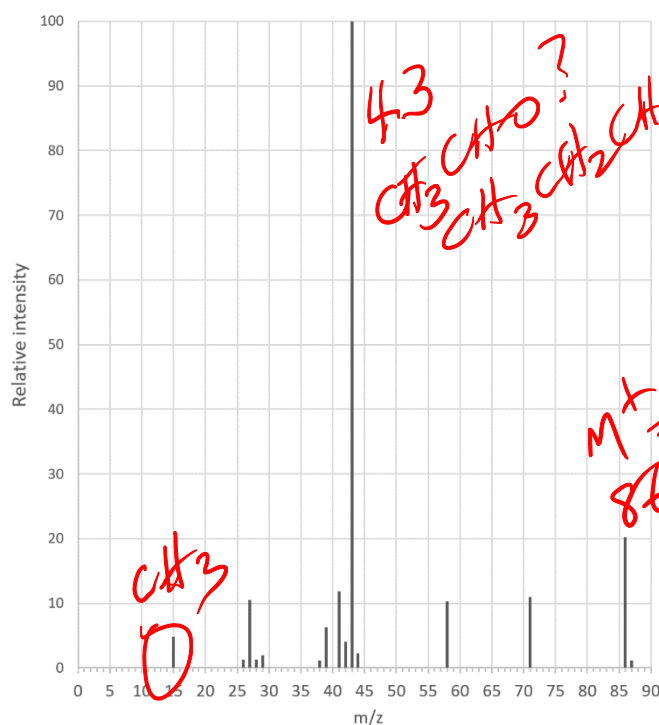
Mass Spectrum
