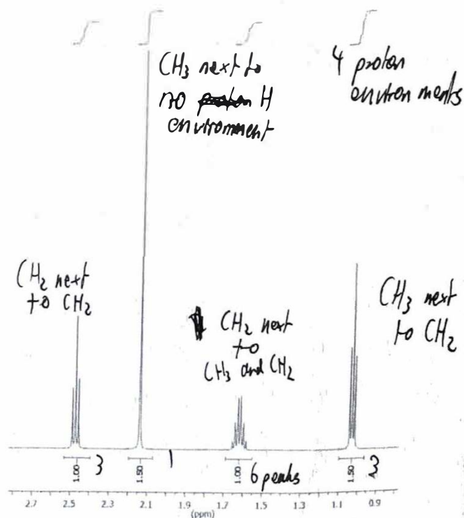
1 H NMR spectrum
